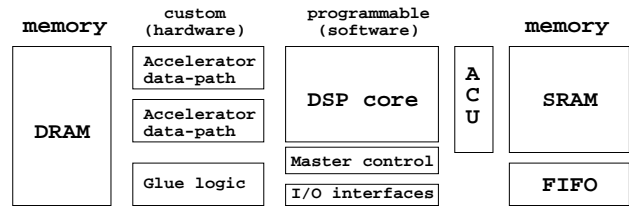
Figure 1: Typical heterogeneous system-on-a-chip architecture for multi-media applications, with custom hardware (application-specific accelerator data-paths and logic), programmable processor (DSP core and controller), and a cost-dominant distributed memory organisation.
